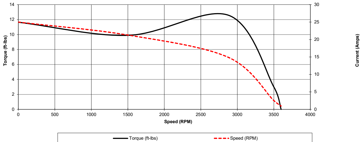
440T, 480T Dual Voltage DOL, 61 leads WYE Connection
